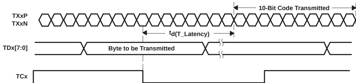
Figure 3–2. Transmitter Latency
